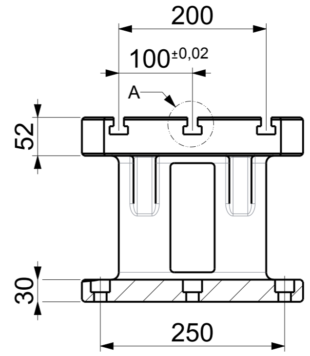
RISER TABLE - T SLOT Art.No. FG/WH/RISTL/TSLOTNP003 Model No. RTT/RT/600300/250-14
