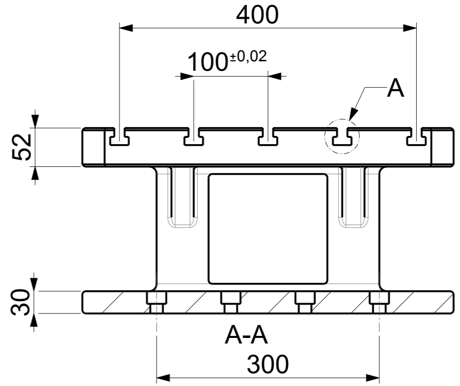
RISER TABLE - T SLOT Art.No. FG/WH/RISTL/TSLOTNP002 Model No. RTT/SQ/500500/250-14
