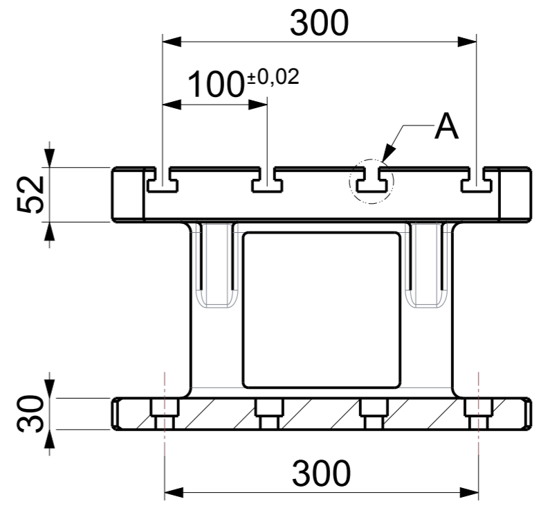
RISER TABLE - T SLOT Art.No. FG/WH/RISTL/TSLOTNP001 Model No. RTT/SQ/400400/250-14
