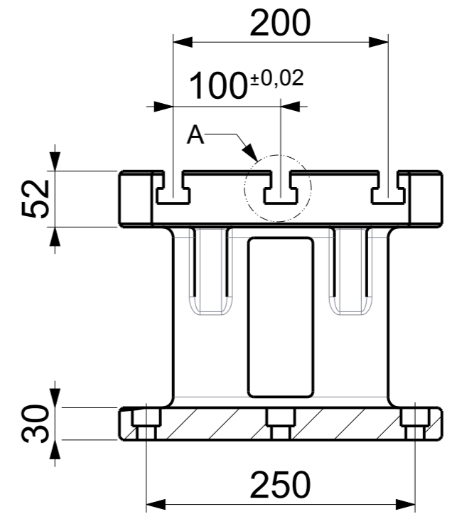
RISER TABLE - T SLOT Art.No. FG/WH/RISTL/TSL18NP003 Model No. RTT/RT/600300/250-18
