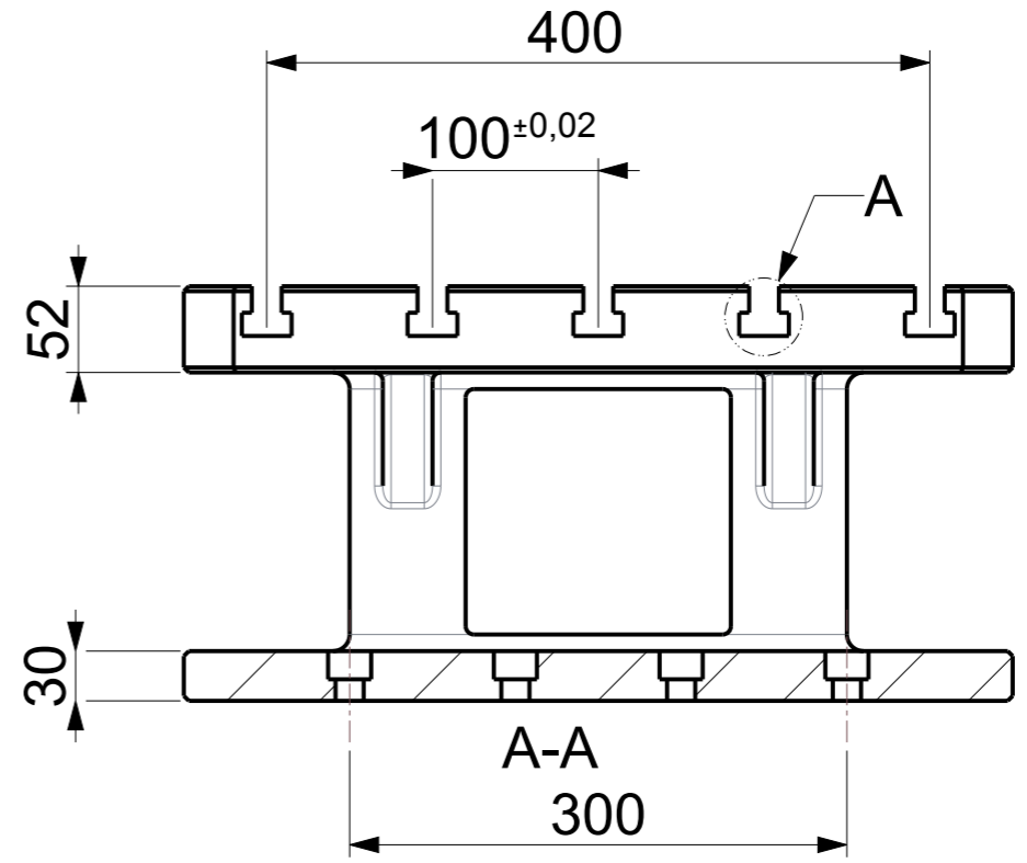
RISER TABLE - T SLOT Art.No. FG/WH/RISTL/TSL18NP002 Model No. RTT/SQ/500500/250-18
