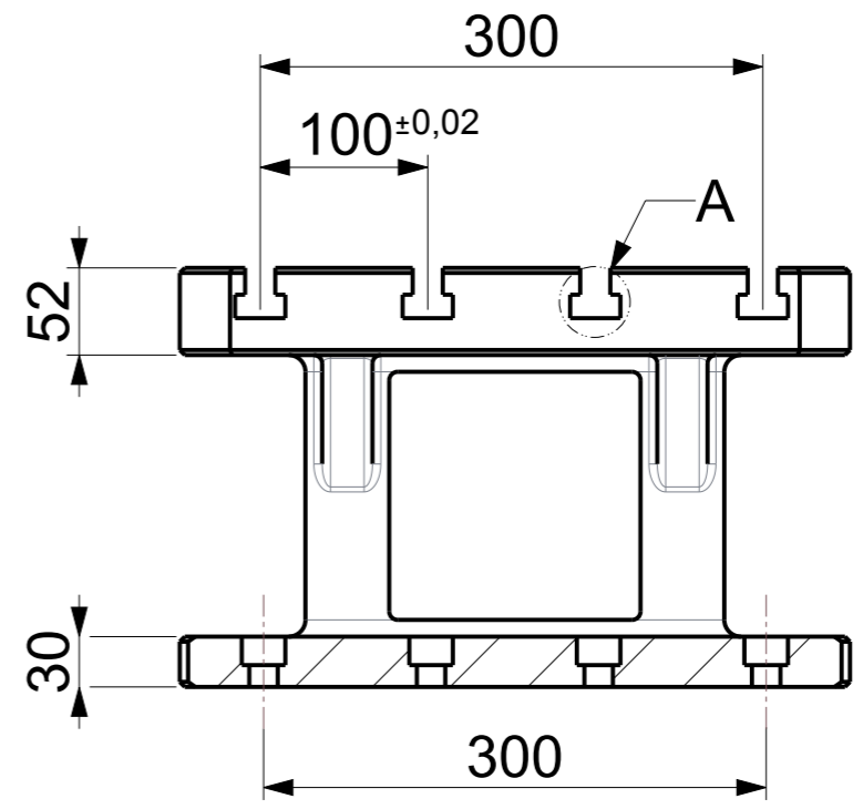
RISER TABLE - T SLOT Art.No. FG/WH/RISTL/TSL18NP001 Model No. RTT/SQ/400400/250-18
