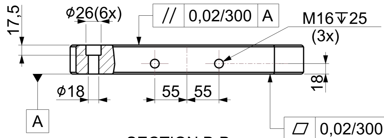
SECTION B-B SCALE 0,250
