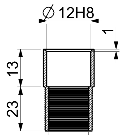
SECTION A-A AFTER INSERT
