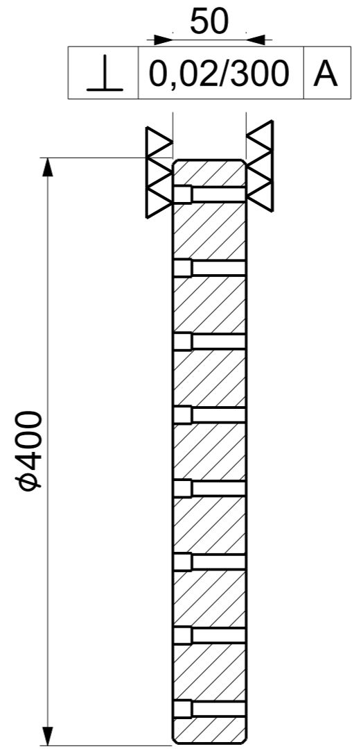
SECTION C-C
