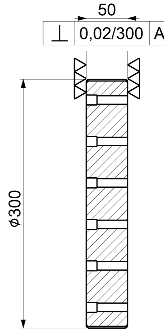
SECTION B-B
