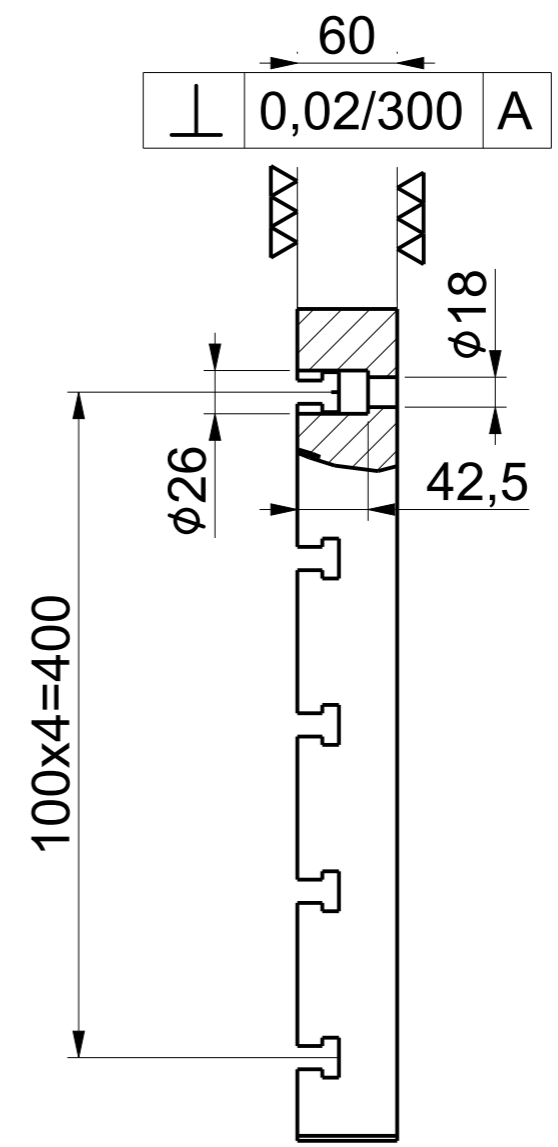
SECTION B-B
