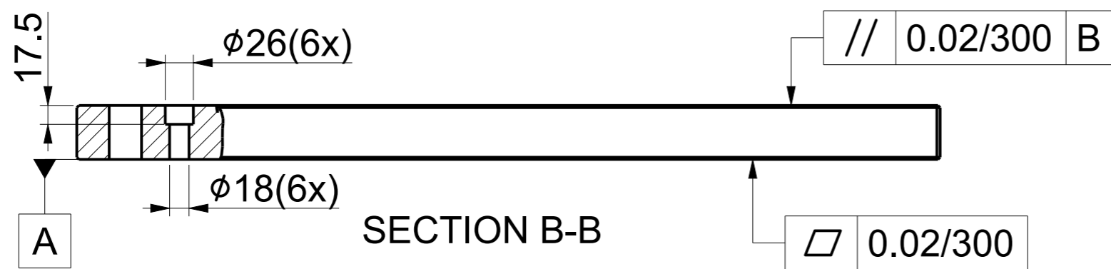
RECTANGULAR BASE PLATE PLAIN Art.No. FG/WH/BASPL/RCPLNNP003 Model.No. BPP/RT/400800
