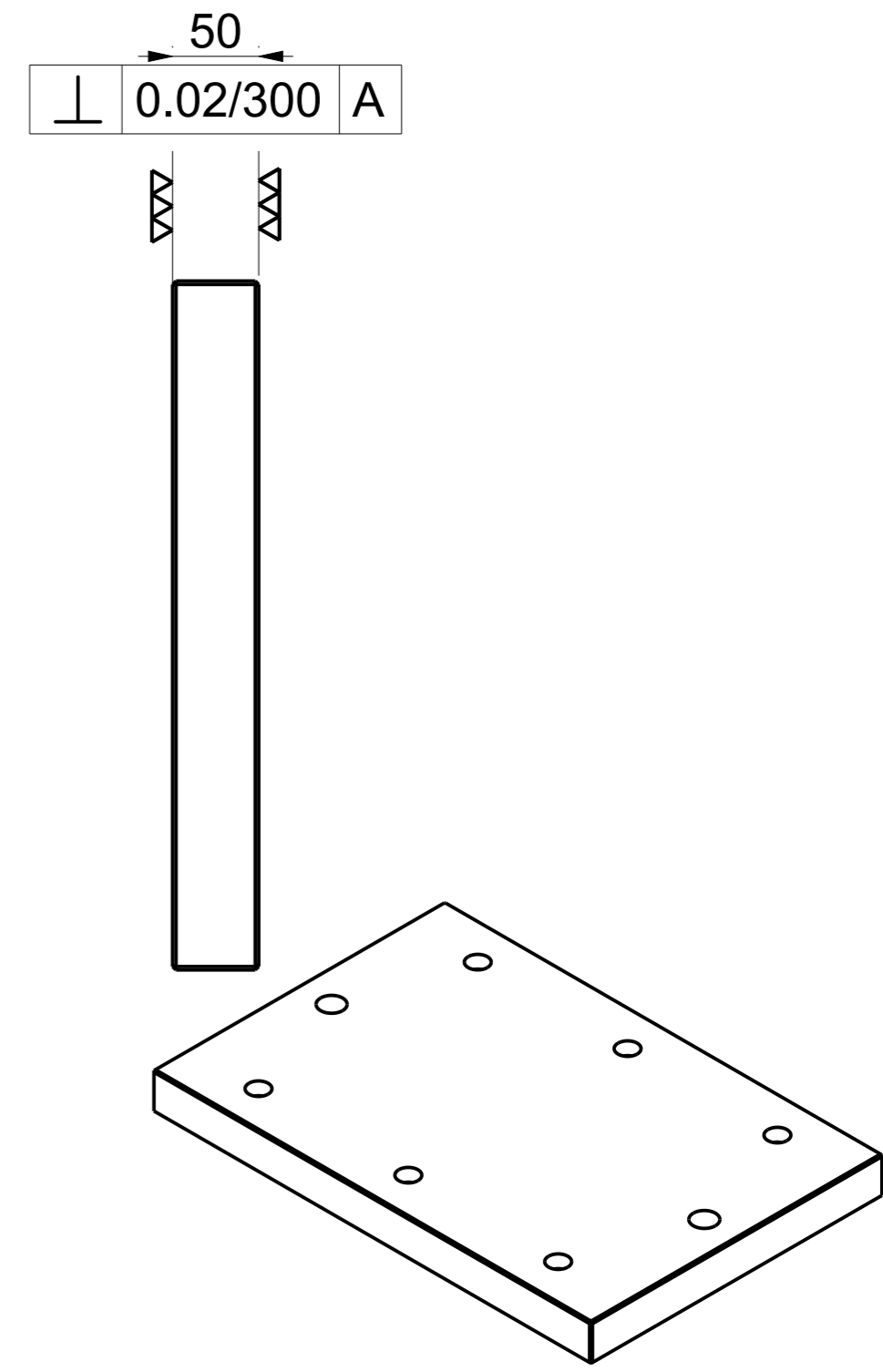
RECTANGULAR BASE PLATE PLAIN Art.No. FG/WH/BASPL/RCPLNNP001 Model No. BPP/RT/400600
