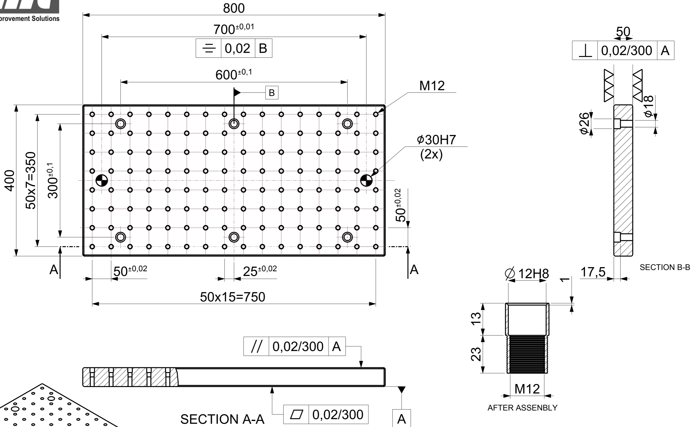
RECTANGULAR BASE PLATE GRID HOLE Art. No. FG/WH/BASPL/RCGRDNP003 Model. No. BPG/RT/400800-12
