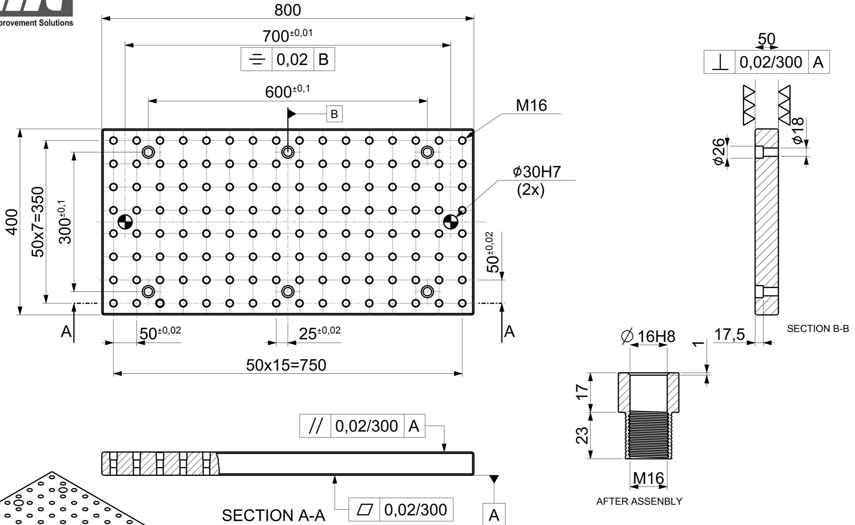
RECTANGULAR BASE PLATE GRID HOLE Art. No. FG/WH/BASPL/RCG16NP03 Model. No. BPG/RT/400800-16
