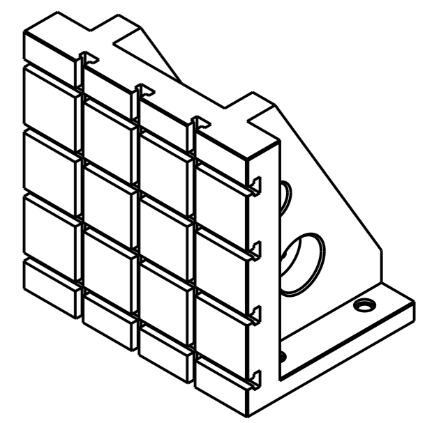
ANGLE PLATE - T SLOT Art.No.FG/WH/ANGPL/ANT14NP001 Model No. APT/SQ/400400-14
