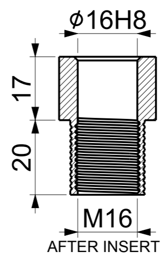
ANGLE PLATE- GRID HOLE Art.No.FG/WH/ANGPL/ANG16NP004 Model No. APG/SQ/800800-16
