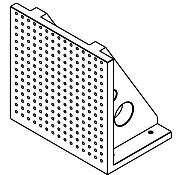
ANGLE PLATE- GRID HOLE Art.No.FG/WH/ANGPL/ANG16NP004 Model No. APG/SQ/800800-16
