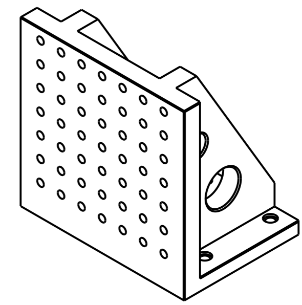
ANGLE PLATE- GRID HOLE Art.No.FG/WH/ANGPL/ANG16NP001 Model No. APG/SQ/400400-16
