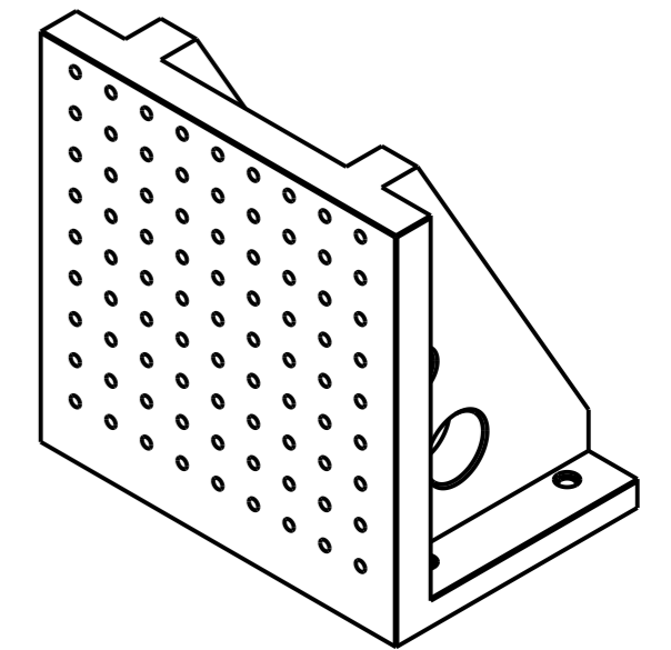
ANGLE PLATE- GRID HOLE Art.No.FG/WH/ANGPL/ANG12NP002 Model No. APG/SQ/500500-12
