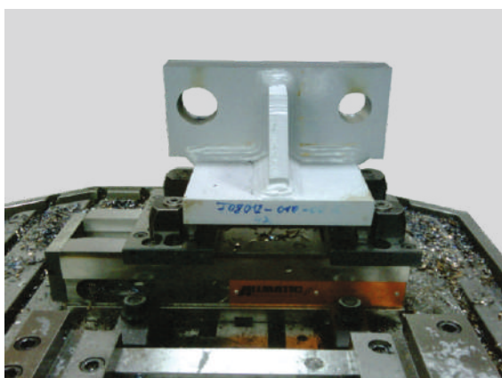
Pivoted Jaws with Universal Gripper
