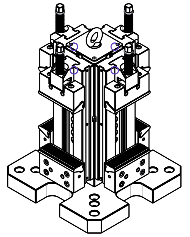
TOMBSTONE 4x90° Art.No. FG/WH/TOMB/SQURENP004 Model. TOMBSTONE 4x90° – MV 150-200
