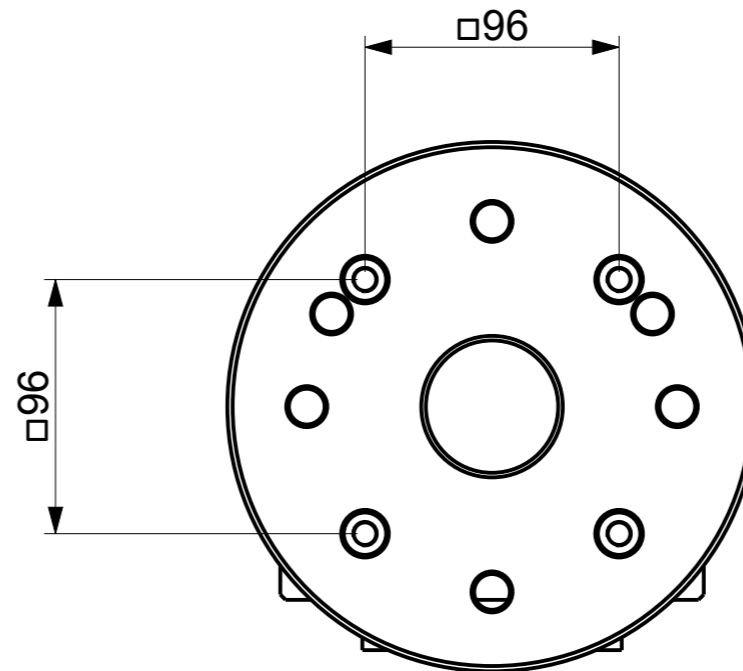
HOLES FOR ZPS
