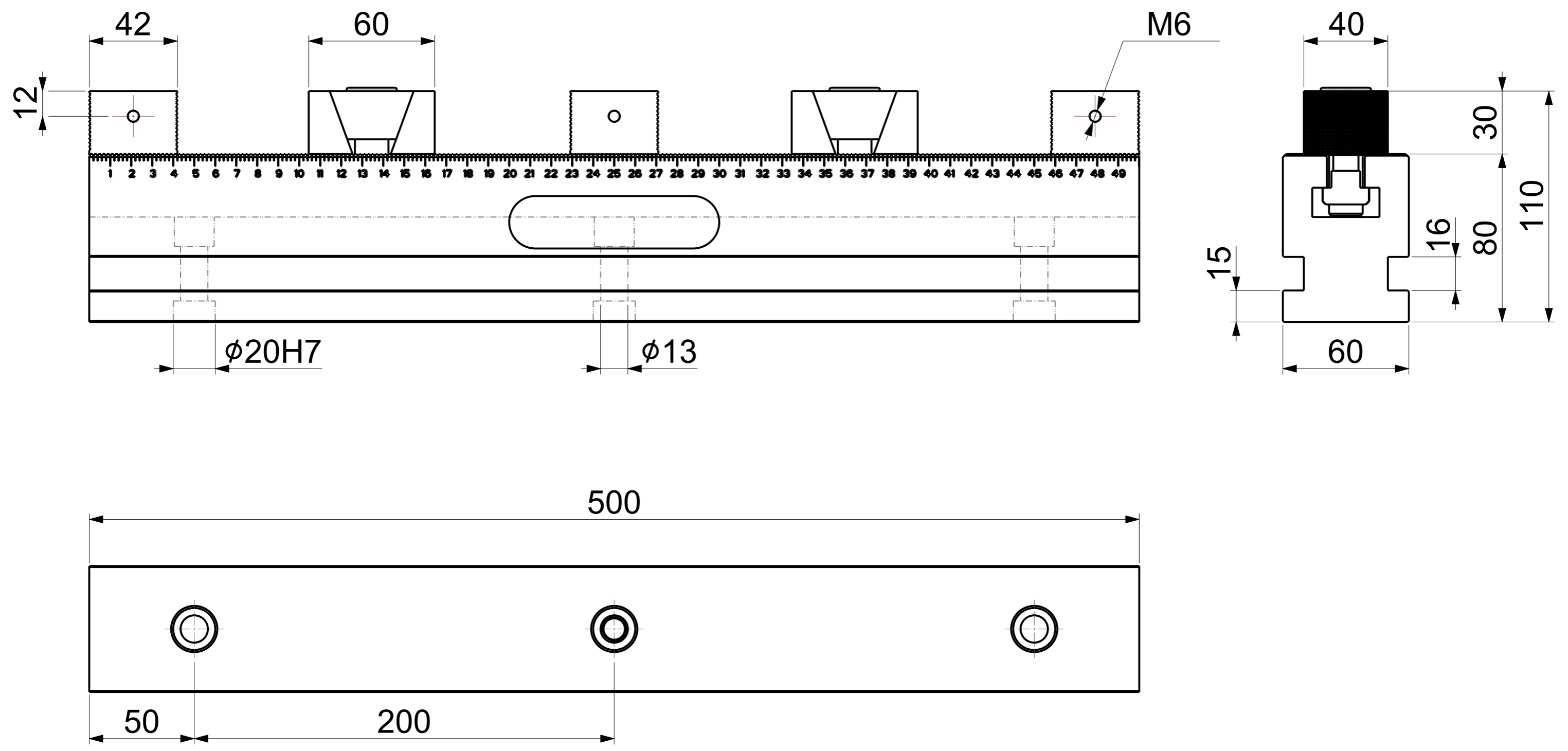
RAIL VISE RL-500 KD-SJ-3 Art.No. FG/VC/RAIL/00500NP002
