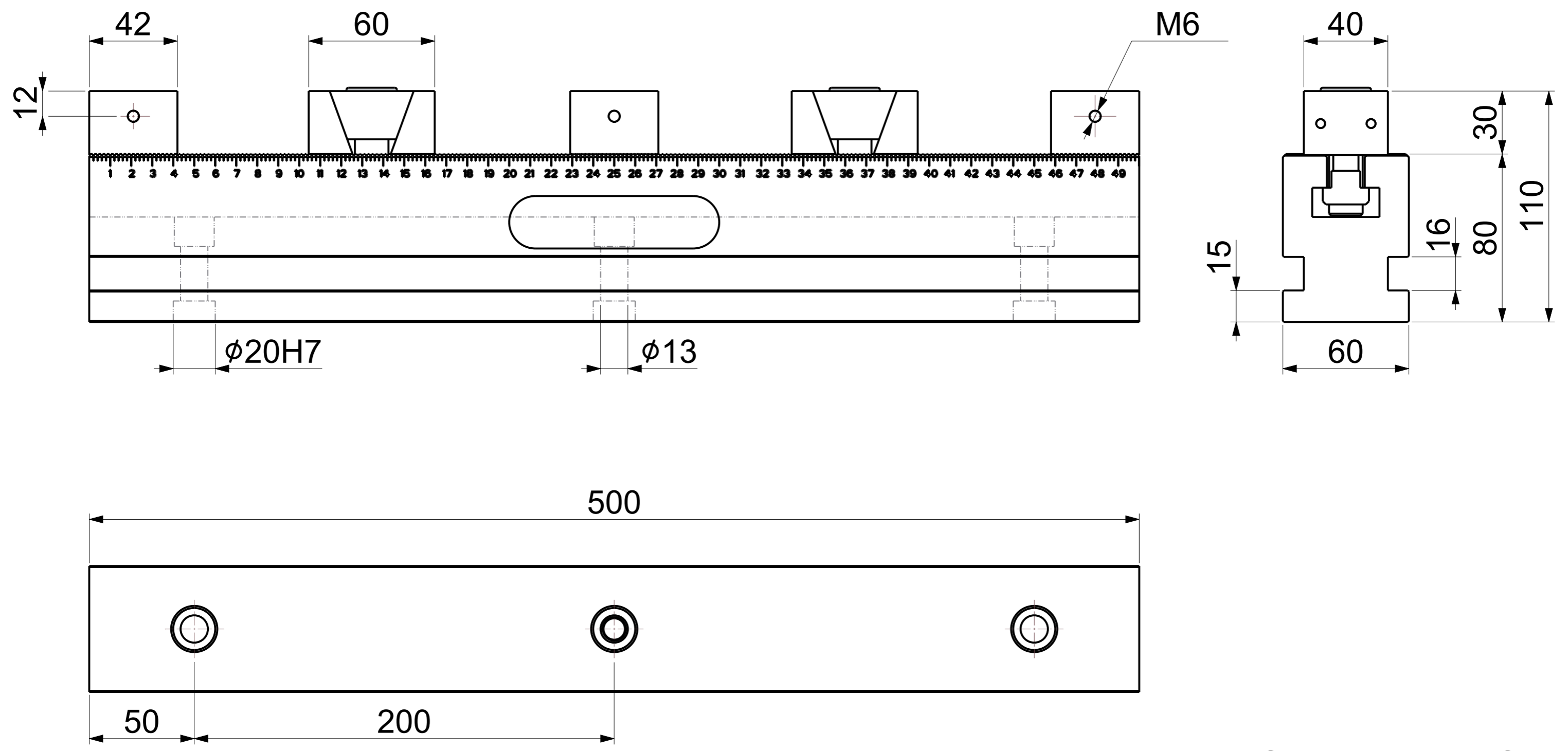
RAIL VISE RL- 500 KD-STJ-3 Art.No. FG/VC/RAIL/00500NP001
