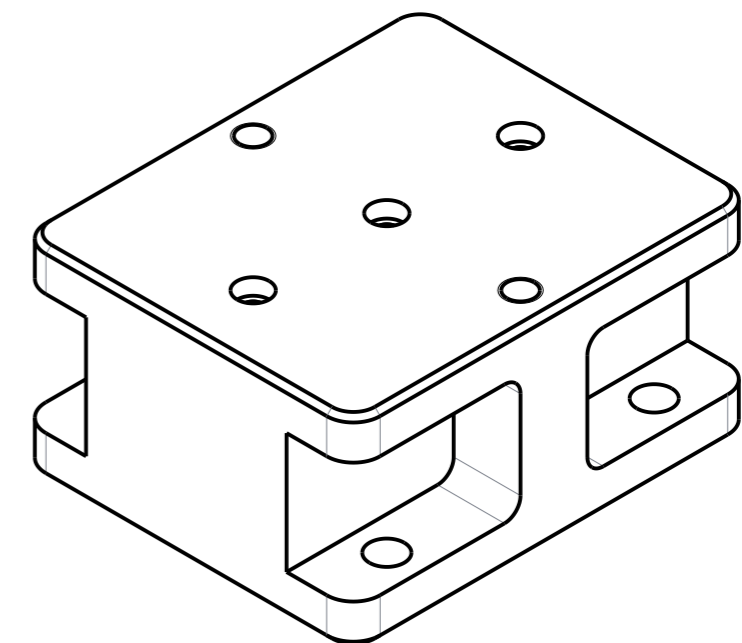
Console SCV 125 Art.No. FG/VC/ACCES/SC014NP001
